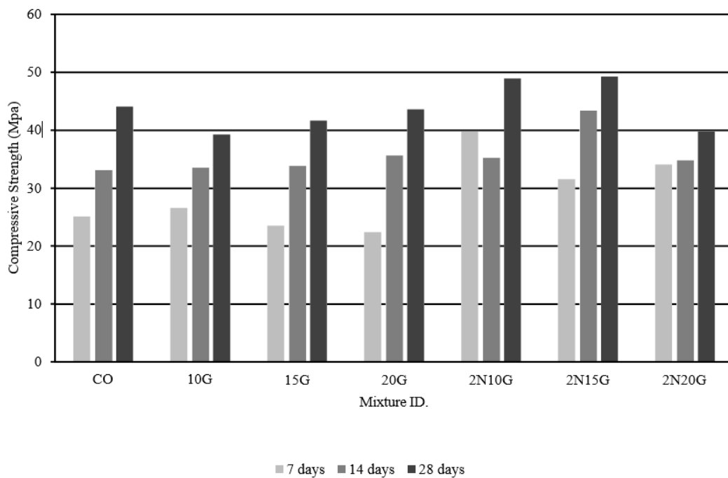
Fig.3 Compressive strength values of samples at 7, 14, and 28 days of curing
