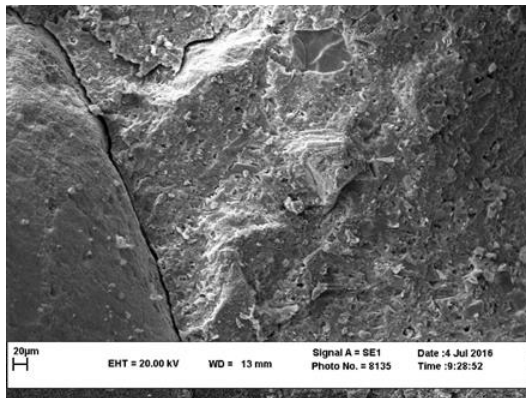
Fig.8.a SEM micrograph of 15G sample – 20 \mu\text{m}
