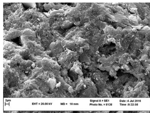
Fig.6.b SEM micrograph of CO sample – 2 µm
