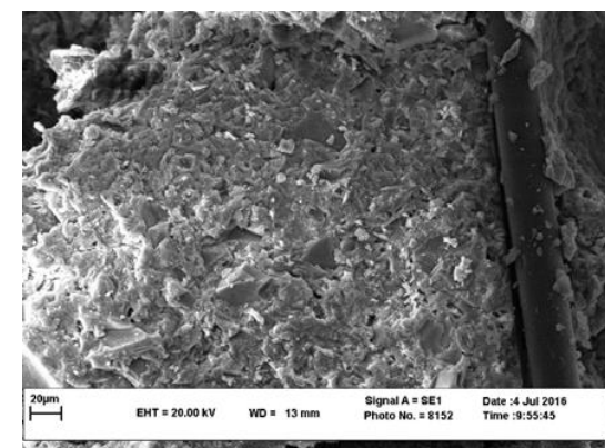
Fig.8.b SEM micrograph of 15G sample – 20 \mu\text{m}
