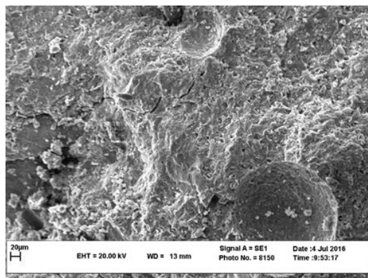
Fig.8.a SEM micrograph of 15G sample – 20 \mu\text{m}
